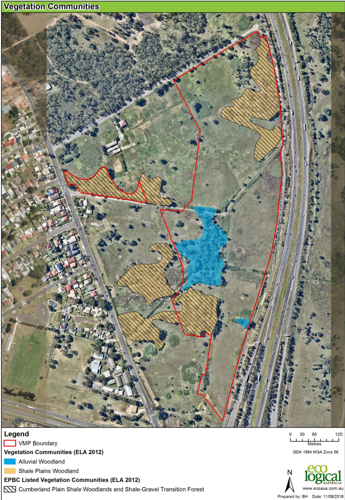
Figure 2: Ecological communities
